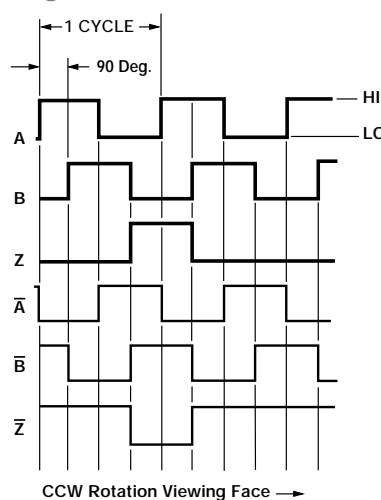
Figure 1 Output Waveform
