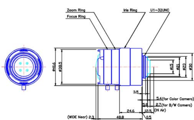
Diagram of Model T3Z2312CS
