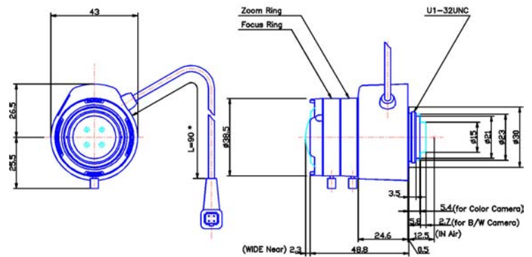
Diagram of Model T3Z2312FCS
